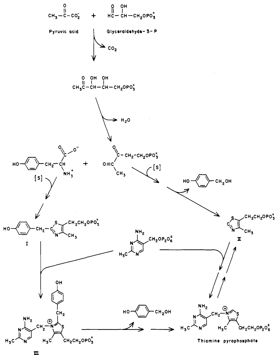
FIGURE 5: Proposed biosynthesis of 4-methyl-5- \beta -hydroxyethylthiazole in E. coli .
